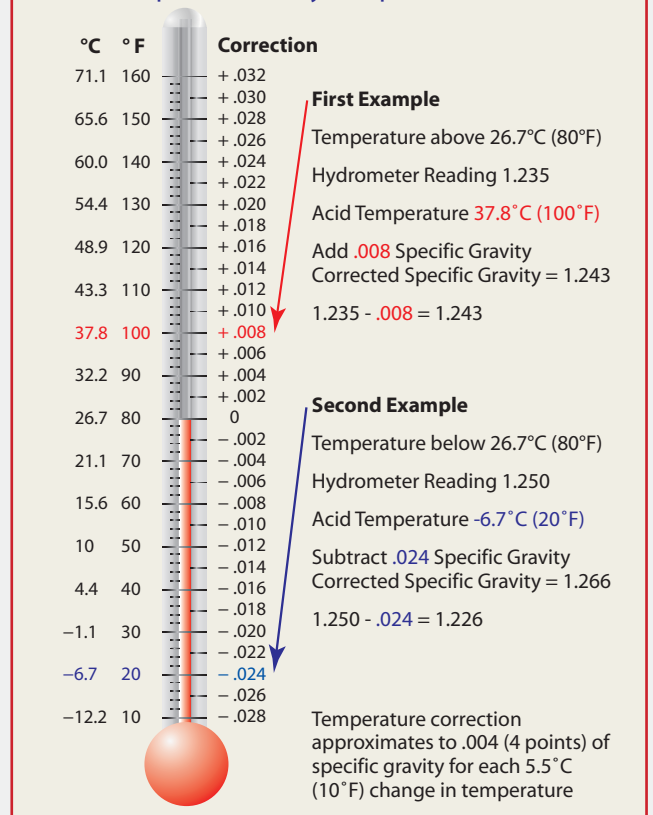
Chart 3- Specific Gravity Temperature Correction
